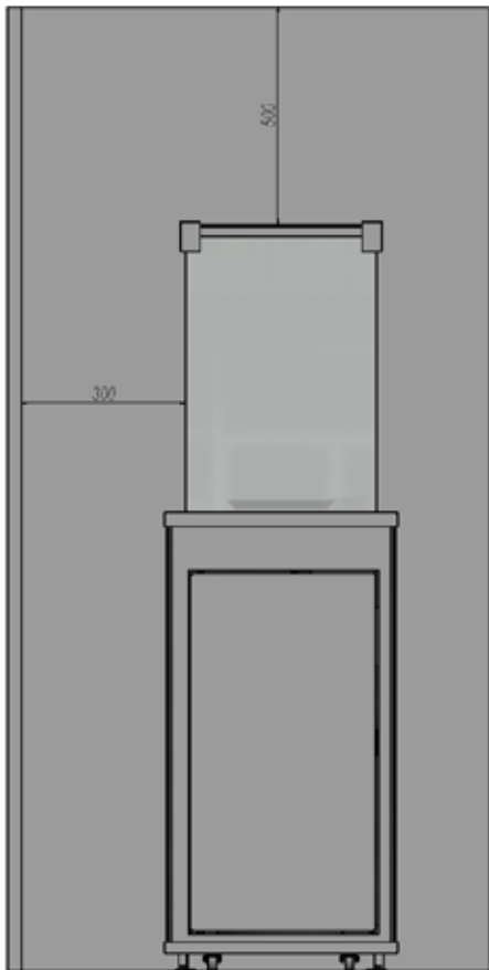
Fig. 4. Minimum distance free from flammable materials
